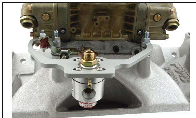
ALL54292 Bracket - Shown With Mallory Regulator
