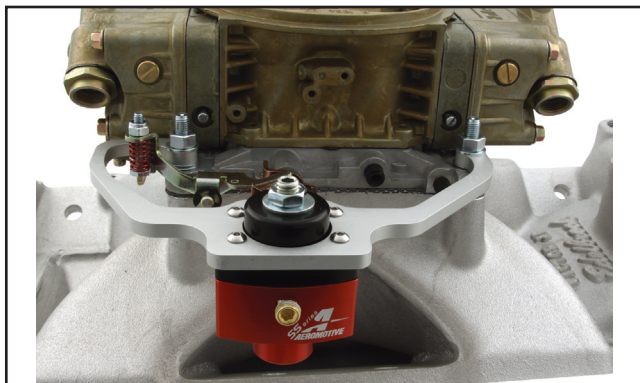
ALL54280 Bracket - Shown With Aeromotive Regulator
